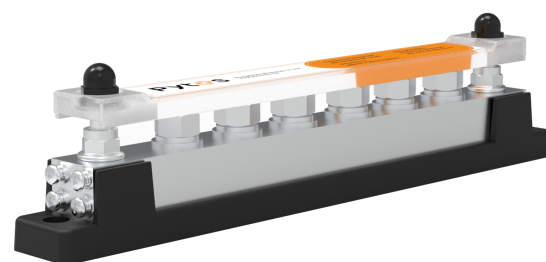
Busbar 600 A 2P with 6 stud terminals and cover
