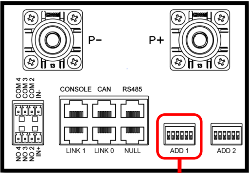
Pi LV1 BCU interface
