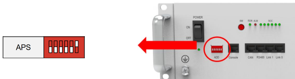
Figure 1.1.4 APS DIP switch setting
