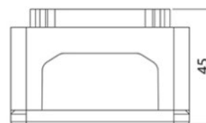
Busbar 300 A 2P with 6 screws and cover (161506100003)
